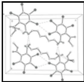
Fig. 2. Part of the crystal structure of (I). Hydrogen bonds are shown as dashed lines.
